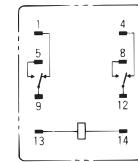
Terminal Arrangement/Internal Connections (Bottom View) Standard Models
